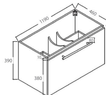
Manu Wall-hung
