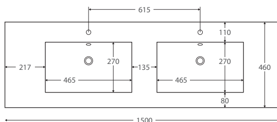
Dolce Vita 1500mm Double Basin
