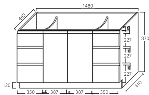
Uni Cabinet with Kick
