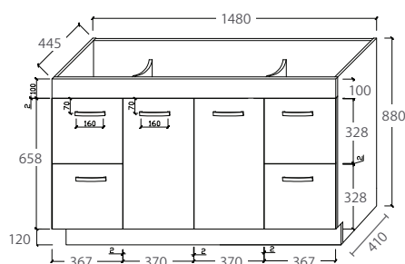
Uni Cabinet with Kick
