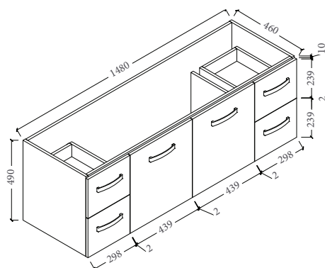
Uni Cabinet Wall Hung
