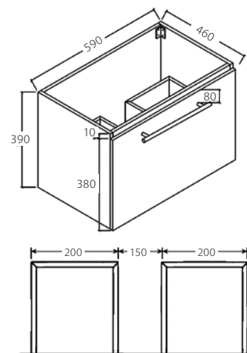
Manu Wall-hung
